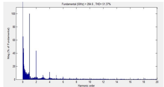
Fig.16: Spectrum of dc side current when n_{z\text{lmt}}=2
