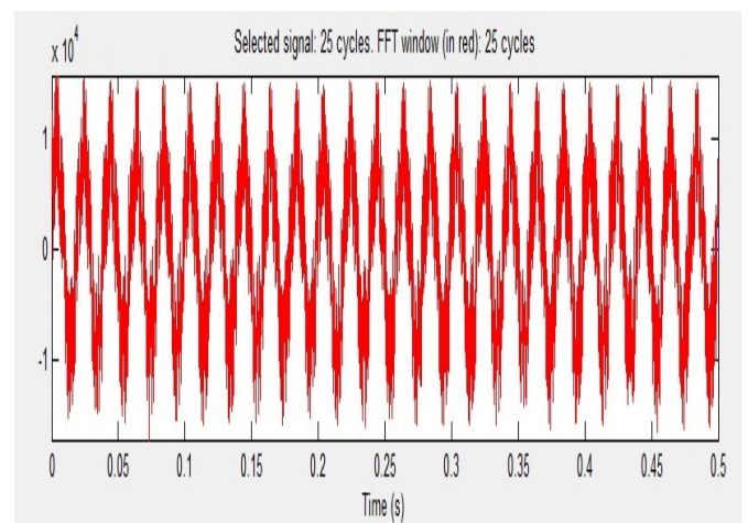
Fig 9: Steady state phase A voltage when n_{zlm}=2
