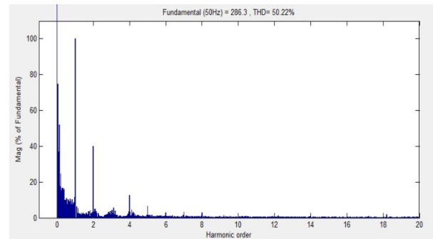
Fig.24: Spectrum of dc side current when n_{z\text{lmt}}=3
