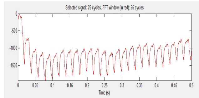
Fig.15: DC side current when n_{z\text{lmt}}=2
