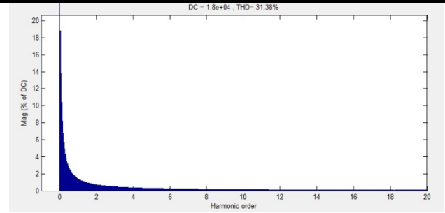
Fig 14: Spectrum of dc side voltage when n_{z\text{lmt}}=2
