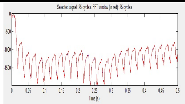
Fig.23: DC side current when n_{z\text{lmt}}=3
