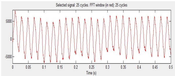
Fig 19: Steady state ac side current when n_{z\text{lmt}}=3
