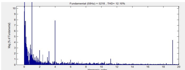
Fig.20: Spectrum of Steady state ac side current when n_{z\text{lmt}}=3
