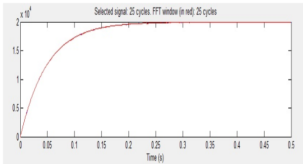
Fig.21: DC side voltage when n_{z\text{lmt}}=3
