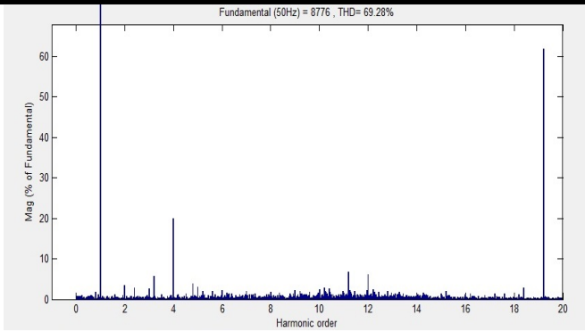
Fig.10: Spectrum of phase A voltage when n_{z\text{lmt}}=2
