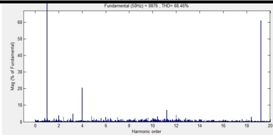
Fig.18: Spectrum of Steady state phase A voltage when n_{z\text{lmt}}=3
