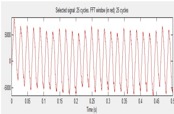
Fig. 11: Steady state ac side current when n_{z\text{lmt}}=2
