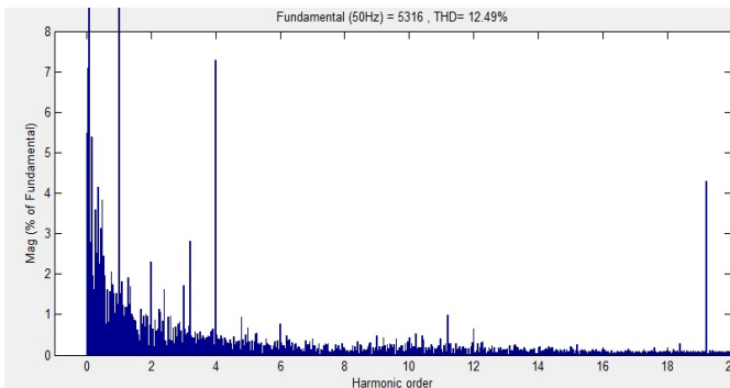
Fig.12: Spectrum of steady state ac side current when n_{z\text{lmt}}=2
