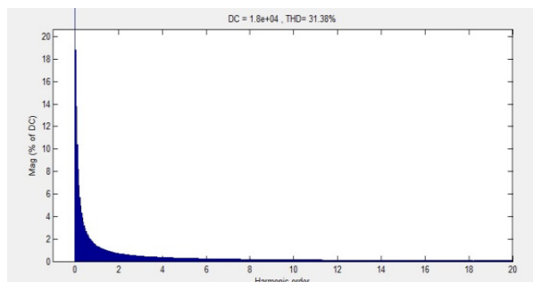
Fig.22: Spectrum of dc side voltage when n_{z\text{lmt}}=3
